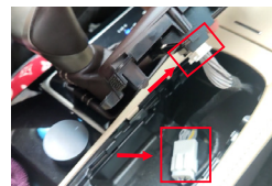
12. Take out the CarPlay knob adapter cable, connect it with the knob plug of the original car, and connect the other end to the knob panel of the original car
