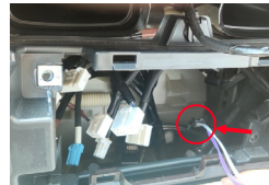
13. Lead the 4PIN plug of the Limcet CarPlay knob adapter cable to the position behind the head unit and connect it to the 4PIN plug on the main line
