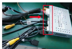
7. Connect the CarPlay main cable and video cable plug to the box, and connect the antenna and USB cable
