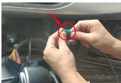
8. Connect iSmart LVDS cable with original car LVDS cable
